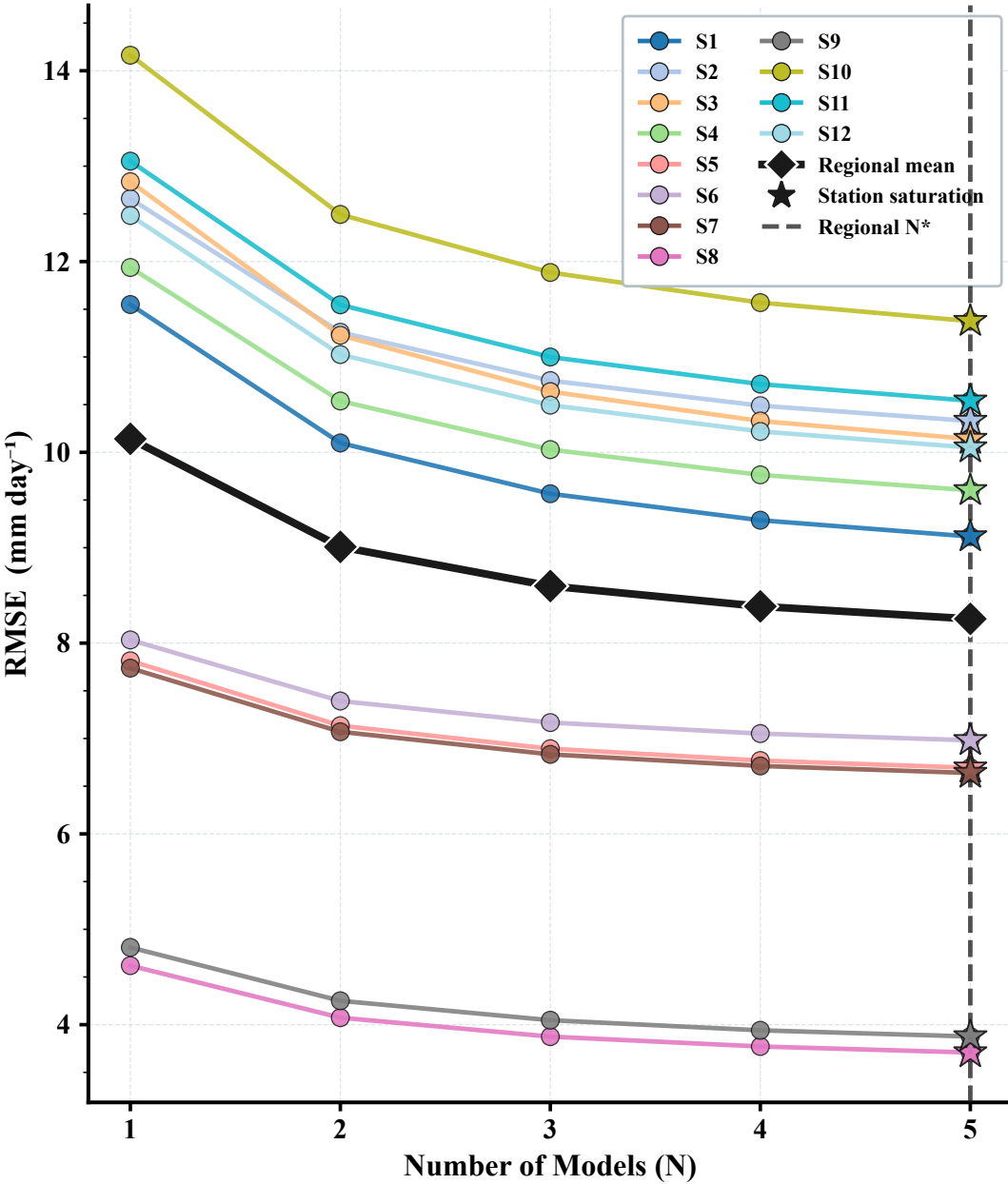
(a) RMSE (mm day -1 ) — Spatial Saturation Each line = one station | = station saturation point Bold line = regional mean
