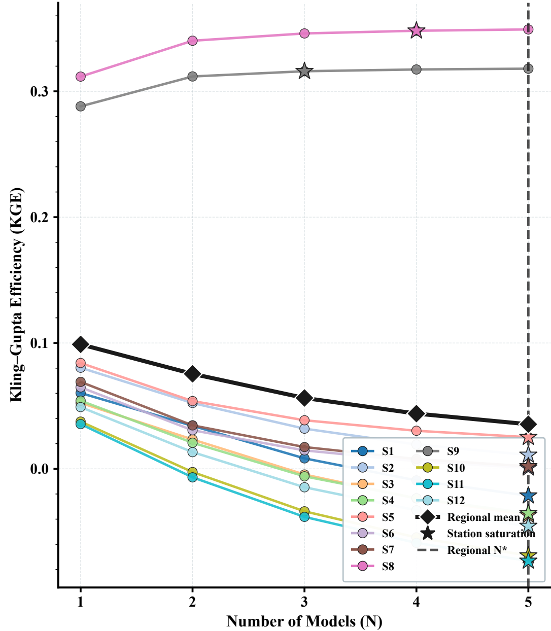
Spatial saturation analysis — Per-station saturation curves (BC QDM) = station saturation point | Dashed line = regional N* | Period: 1981–2014 (b) Kling–Gupta Efficiency (KGE) — Spatial Saturation Each line = one station | = station saturation point Bold line = regional mean
